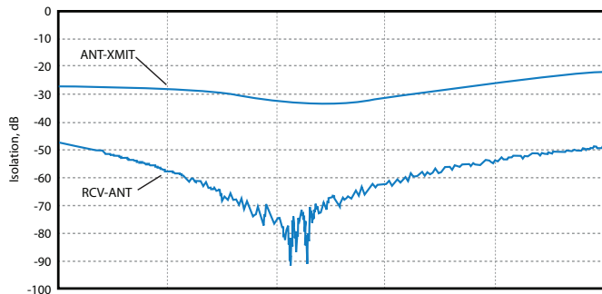
Typical Isolation
