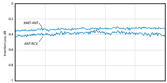
Typical Insertion Loss
